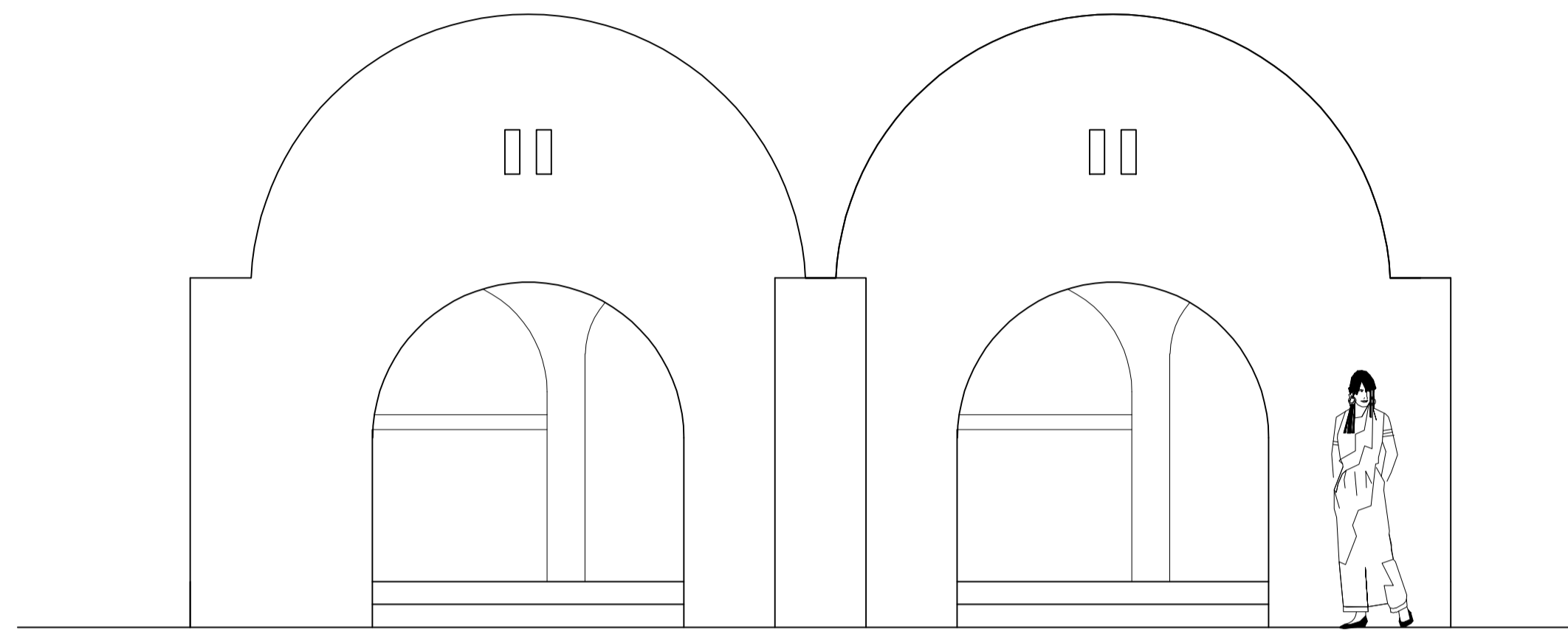
Façade Principale
